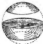
SEGMENT SFERIC
