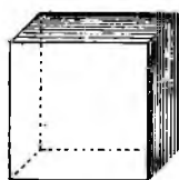
EXAEDRU (CUB)
