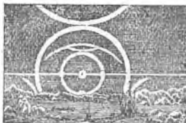
Fig. 3582a. Parhelie.
